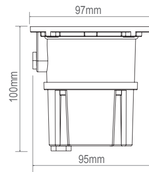
LED body
